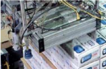
Side clamp tooling works well with thinner-walled sustainable packaging, and offers flexibility for packaging lines that run a variety of products.
